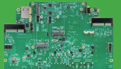
NBC-3003 - Supports Jetson Thor - 5G, 4G, Wi-Fi - 3 × USB3.0, 3 × LAN - 1 × COM, 2 × CAN - 6 × Antennas
