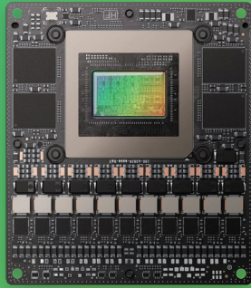
Jetson Thor T5000 2070 TFLOPS 40 ~ 130 W
