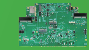
NBC-3003 - Supports Jetson Thor - 5G, 4G, Wi-Fi - 3 × USB3.0, 3 × LAN - 1 × COM, 2 × CAN - 6 × Antennas
