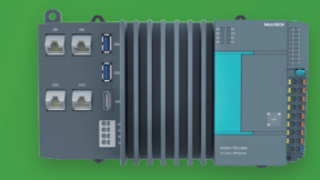
MX 6000 Series - Supports Jetson Orin Nano - Connects AI, OT, and IT. - Providing customers with edge-layer automation processing capabilities and data acquisition, analysis, storage, and other capabilities.
